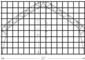
30' (9.1m) Meridian Outside Width: 30' (9.1m) Outside Height: 18' 7 1/2" (5.6m) Maximum Clearance: 16' 9 1/2" (5.1m)
