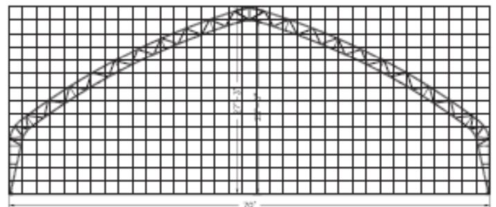
70' (21.3m) Meridian Outside Width: 70' (21.3m) Outside Height: 27' 3" (8.3m) Maximum Clearance: 25' 5" (7.7m)
