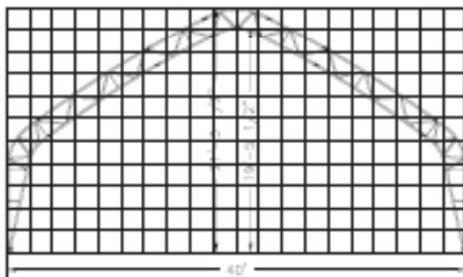
40' (12.1m) Meridian Outside Width: 40' (12.1m) Outside Height: 21' 3 1/2" (6.4m) Maximum Clearance: 19' 5 1/2" (5.9m)
