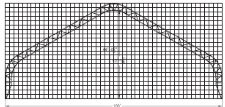
100' (30.4m) TITAN Outside Width: 100' (30.4m) Outside Height: 44' 0 1/2" (13.4m) Maximum Clearance: 40' 9 1/4" (15.1m)
