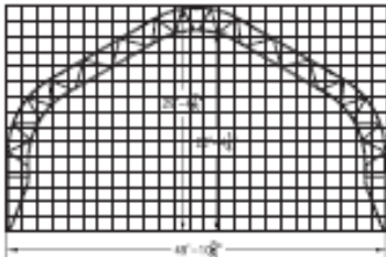
50' (15.2m) TITAN Outside Width: 49' 10 1/8" (15.2m) Outside Height: 29' 7 3/4" (9.0m) Maximum Clearance: 26' 3 1/4" (8.0m)
