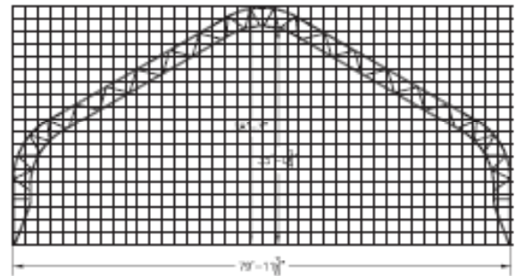
80' (24.3m) TITAN Outside Width: 79' 11 1/8" (24.3m) Outside Height: 38' 3" (11.6m) Maximum Clearance: 35' 0 3/8" (10.6m)
