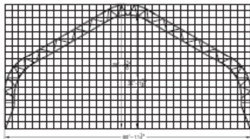
70' (21.3m) TITAN Outside Width: 69' 11 1/8" (21.3m) Outside Height: 35' 4 3/8" (10.7m) Maximum Clearance: 32' 1 3/4" (9.7m)
