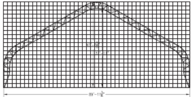
90' (27.4m) TITAN Outside Width: 89' 11 1/8" (27.4m) Outside Height: 41' 1 1/4" (12.5m) Maximum Clearance: 37' 11" (11.5m)
