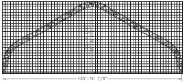
130' (39.6m) TITAN Outside Width: 130' 10 7/8" (39.9m) Outside Height: 52' 4 1/2" (15.9m) Maximum Clearance: 48' 5 1/2" (14.7m)
