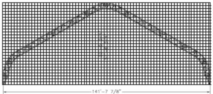
140' (42.6m) TITAN Outside Width: 141' 7 7/8" (43.1m) Outside Height: 55' 5 1/4" (16.9m) Maximum Clearance: 51' 6 1/4" (15.7m)
