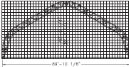
90' (27.4m) TITAN Outside Width: 89' 10 1/8" (27.3m) Outside Height: 40' 6 1/4" (12.3m) Maximum Clearance: 36' 7 1/4" (11.1m)
