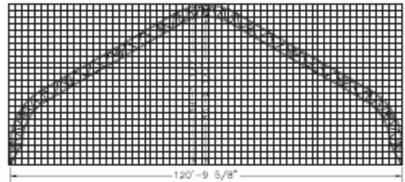
120' (36.5m) TITAN Outside Width: 120' 9 5/8" (36.8m) Outside Height: 49' 5 1/2" (15.0m) Maximum Clearance: 45' 6 1/2" (13.8m)
